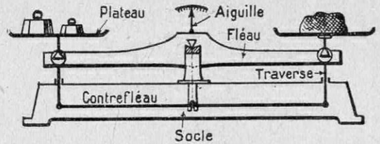
FIG. 8. — BALANCE ROBERVAL
